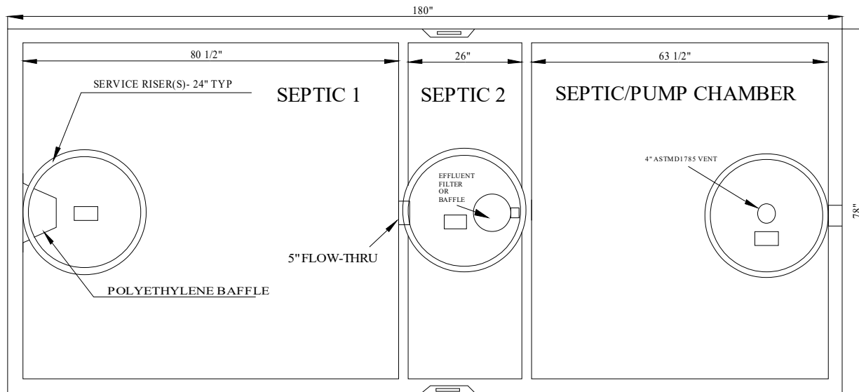
TOP VIEW
