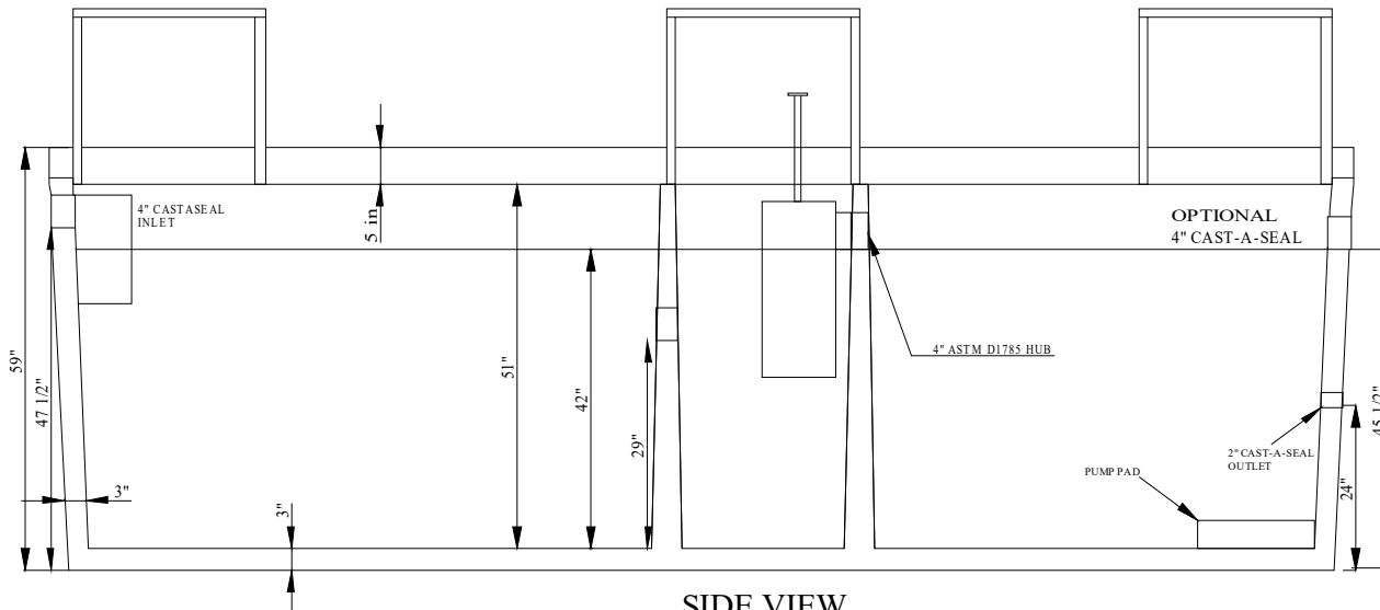
SIDE VIEW
